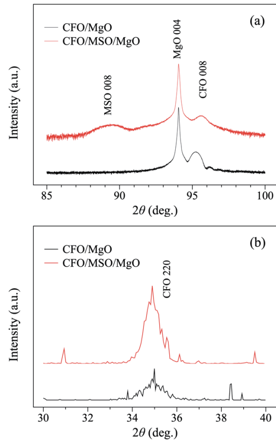
Fig. 2 XRD patterns of CFO/MgO and CFO/MSO/MgO. (a) Out-of-plane patterns in range of 85 – 100°, (b) In-plane patterns in range of 30 – 40°.
