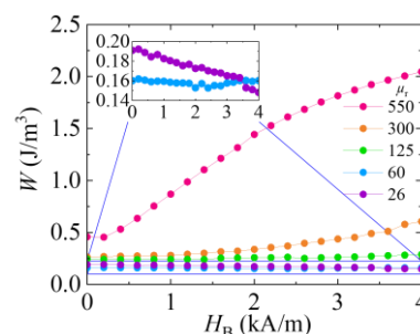
Fig. 1. Bias dependence of iron loss of Mo permalloy with different \mu_r .
