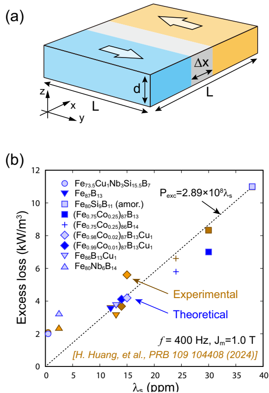
Fig 1: (a) Simple stripe domain mode for our formulation. (b) Excess losses obtained by experimental and theoretical calculations.
