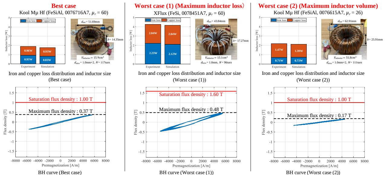
Fig. 2 Example of optimal design results for AC filter inductor
