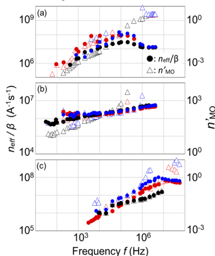
Fig.2 Effective domain wall number over the domain wall damping n_{\text{eff}}/\beta (circle) and effective active MOs number n'_{\text{MO}} (triangle) of (a) Mn-Zn ferrite sintered, (b) FINEMET wound, and (c) Sendust powder cores for B_m = 1 mT (blue), 10 mT (red), and 100 mT (black) as a function of frequency.
