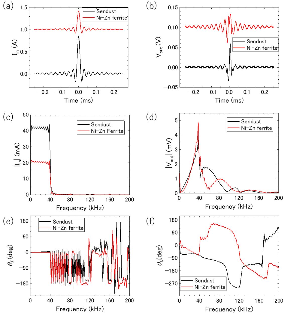
Fig.1 (a, b) Measured (a) I_{in} and (b) V_{out} . (c-e) Fourier transformed results of the measured I_{in} and V_{out} . Black and red lines indicate the results of Sendust and Ni-Zn ferrite, respectively.
