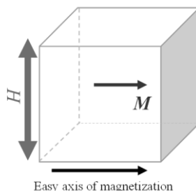
Fig.1 Single domain model.
