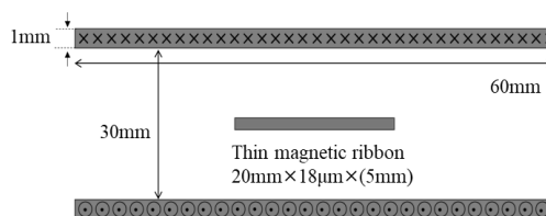
Fig.3 Ribbon model for Maxwell simulation.
