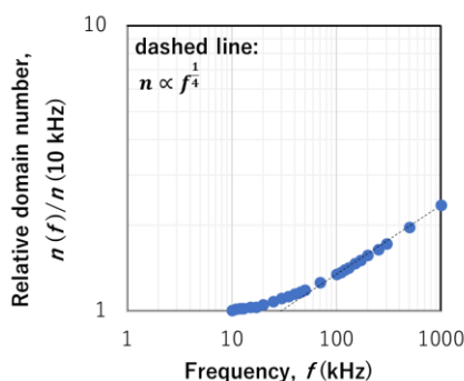
Fig. 1 Frequency dependence of domain number.
