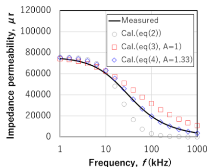
Fig. 2 Frequency dependence of permeability.
