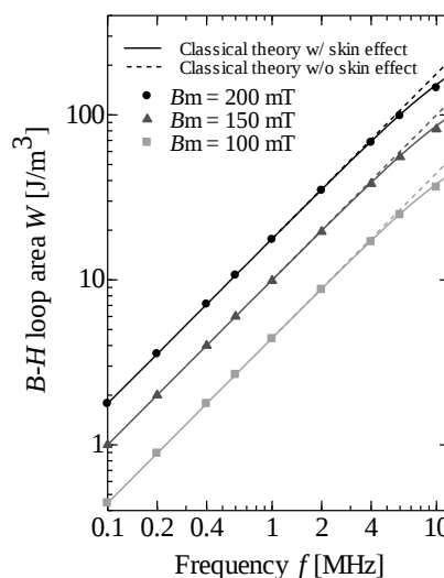
Fig.1 Dynamic loss vs. frequency obtained from LLG/Maxwell simulation.
