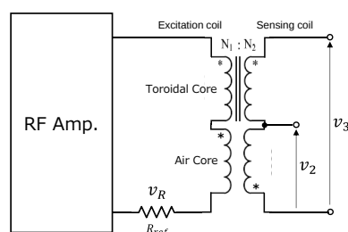
Fig.2 Inductive Cancellation Method
