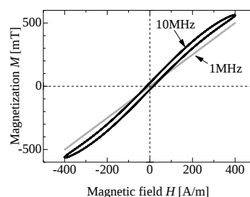
Fig. 2 Dynamic M-H loop obtained from LLG analysis.
