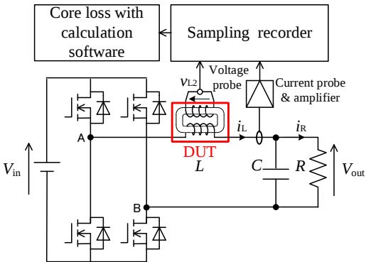
Fig. 1 Single-phase PWM inverter circuit
