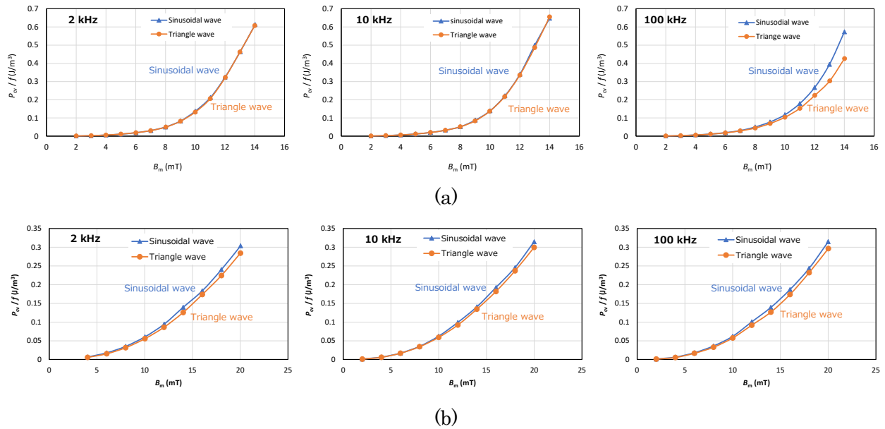
Fig.4 Comparison between sinusoidal and triangle waveform excitation. The measurement frequencies are 2 kHz to 100 kHz. (a) Ferrite core and (b) Sendust dust core.
