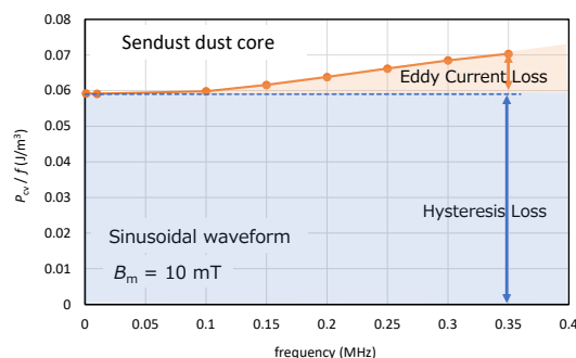
Fig.3 Frequency dependence of core loss of Sendust dust core
