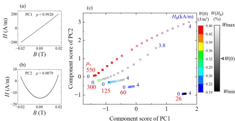
Fig. 2. PCA results for magnetic score with different magnetic permeability. (a) Principal component PC1, (b) Principal component PC2, (c) Principal component score of PC1 and PC2. Note: Wmin = 80, Wmax = 120 at \mu_r = 26, 60, 125 and 300. Wmax = 500 at \mu_r = 550 (Only Wmax is defined).
