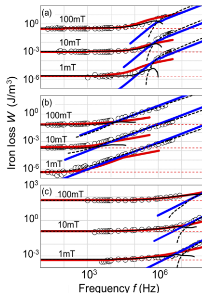
Fig.1 Iron loss per cycle obtained by experiments (marks) and analysis (lines) of (a) Mn-Zn ferrite sintered, (b) FINEMET wound, and (c) Sendust powder cores.
