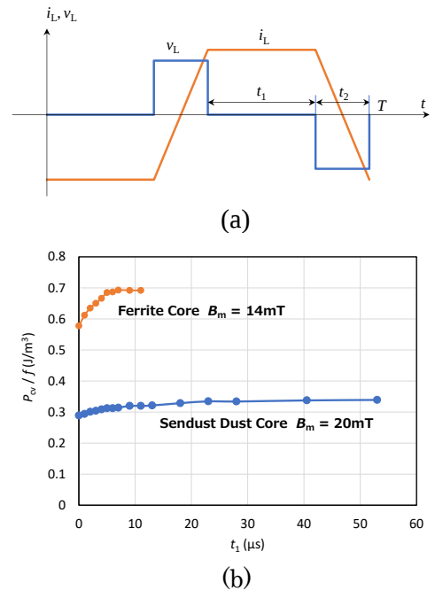
Fig.5 (a) Trapezoidal current waveform for measuring magnetic relaxation. (b) Measurement results of magnetic relaxation.
