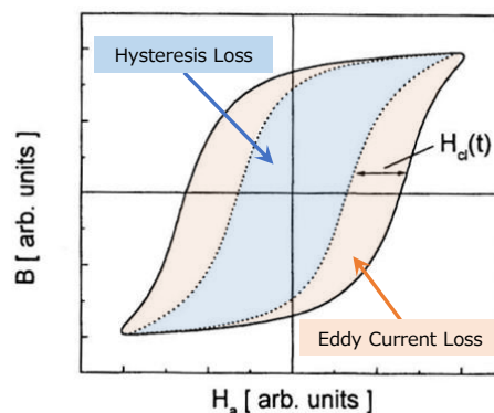
Fig.1 Hysteresis loop shape (1)
