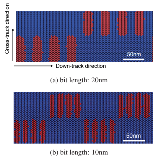
Fig. 2 Printed magnetization distributions of burst signals with bit lengths of (a) 20 nm and (b) 10 nm.
